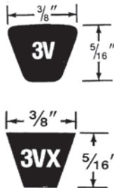
“3V & 3VX” V-Belts
